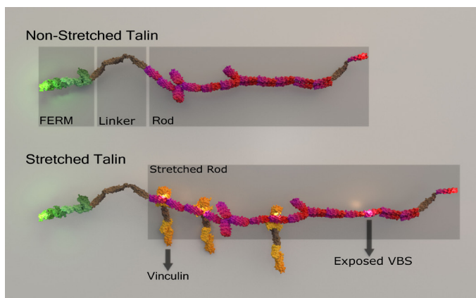
Figure: Talin stretching and stretch-induced vinculin binding
